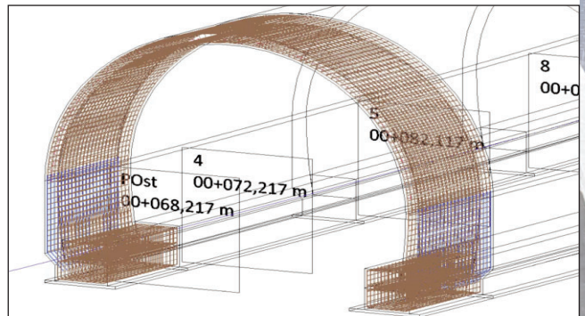
SOFiSTiK Bridge + Infrastructure Modeler: Tunnel Bewehrung/Reinforcement
